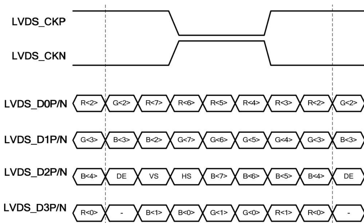
8-bit LVDS input_JEDIA format
